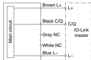
When used as an IO-Link device
