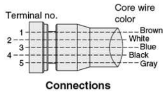
Connections
