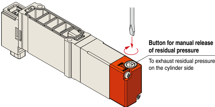
Exhaust center
