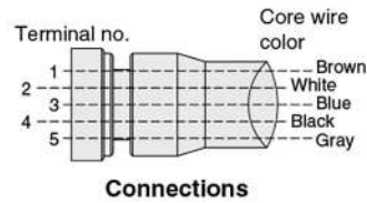
Connections
