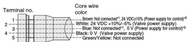
Connections (DeviceNet®, EtherNet/IP™)
