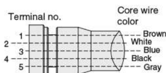
Connections
