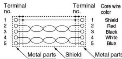
Connections
