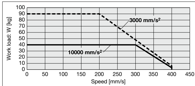
Horizontal/Lead 8
