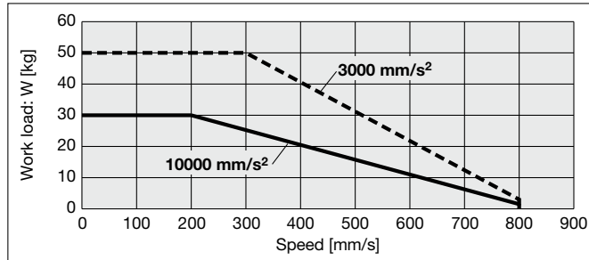
Horizontal/Lead 16
