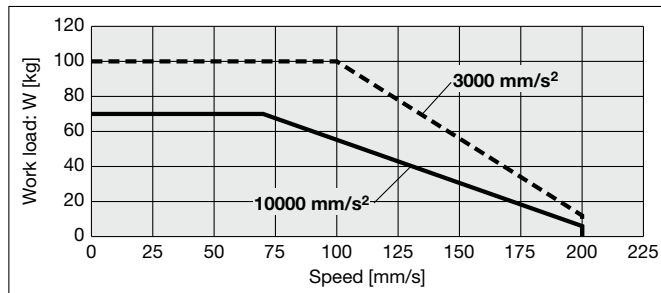
Horizontal/Lead 4
