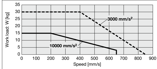
Horizontal/Lead 24
