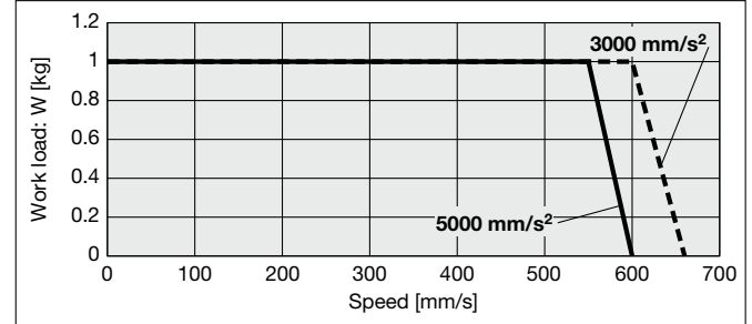
Vertical/Lead 24
