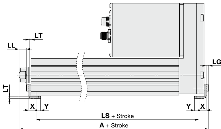
Outward mounting
