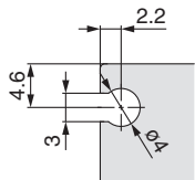
Dimensions of auto switch mounting groove
