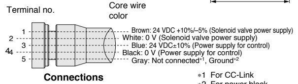
Socket connector pin arrangement B-coded (Reverse key)
