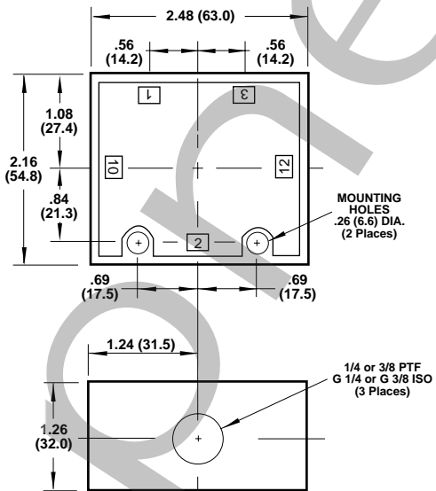
3-WAY - 1/4" & 3/8" PORTS K41
