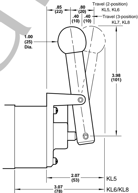
KL5/KL8 – LEVER
