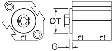
Front Boss - Ø20 - Ø25 Bores
