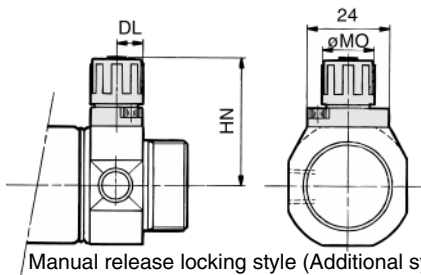
Manual release locking style (Additional symbol: L)
