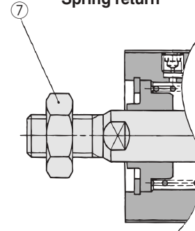
Spring return
