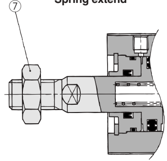
Spring extend
