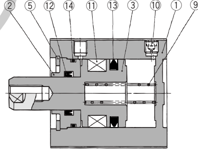
Spring return
