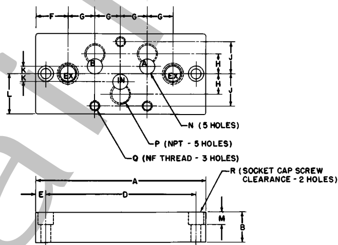
BOTTOM PORTED
