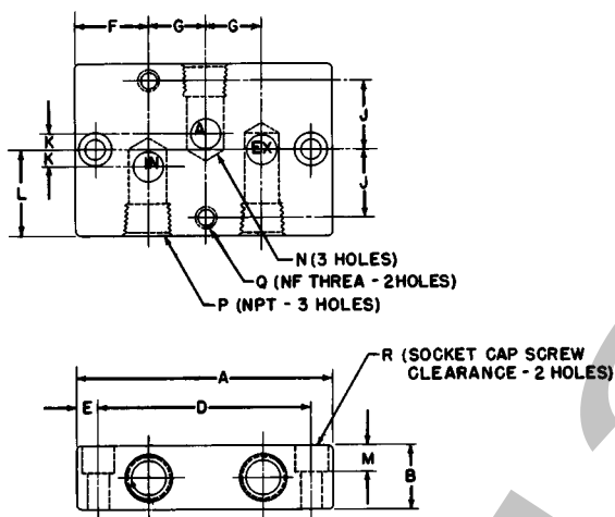
SIDE-PORTED
