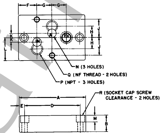
BOTTOM PORTED
